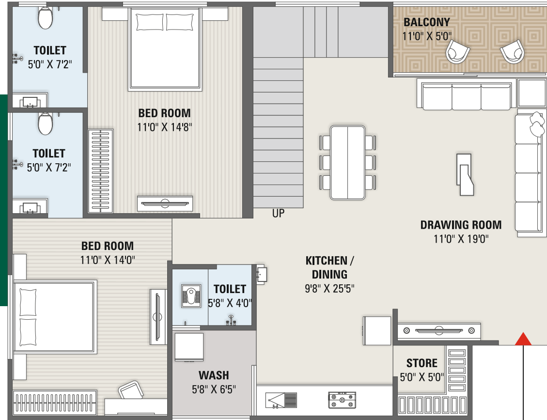
12th Floor Penthouse Lower Level Plan
